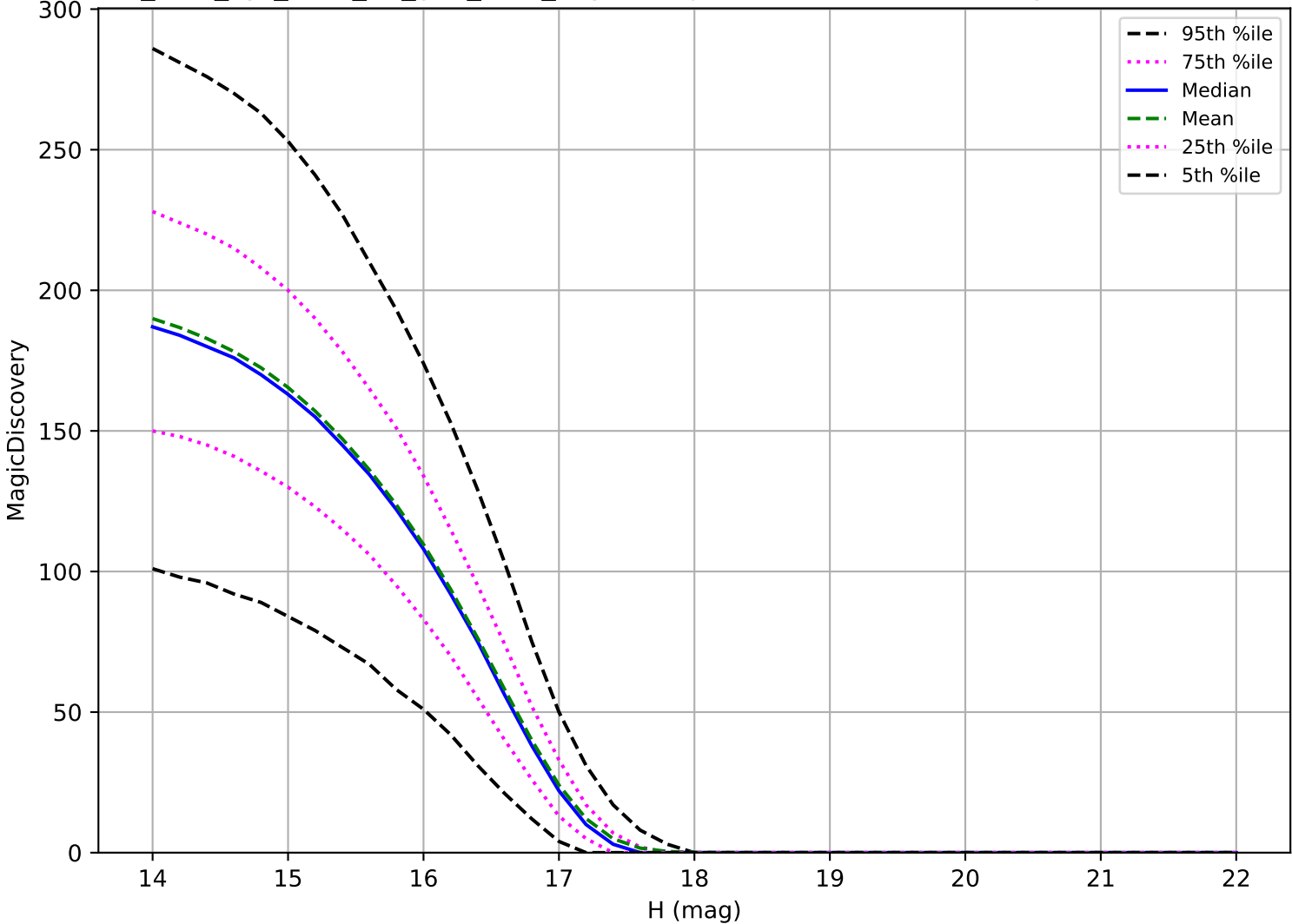
too_elab_2yr_r128_d2_griz_v3.4_10yrs: Trojan 6 detections in 60 nights detection loss
