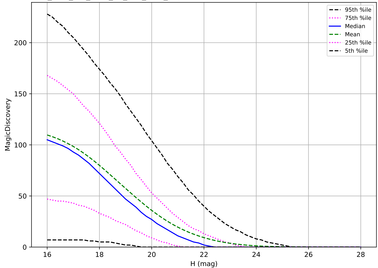
too_elab_2yr_r128_d2_griz_v3.4_10yrs: PHA 6 detections in 60 nights detection loss
