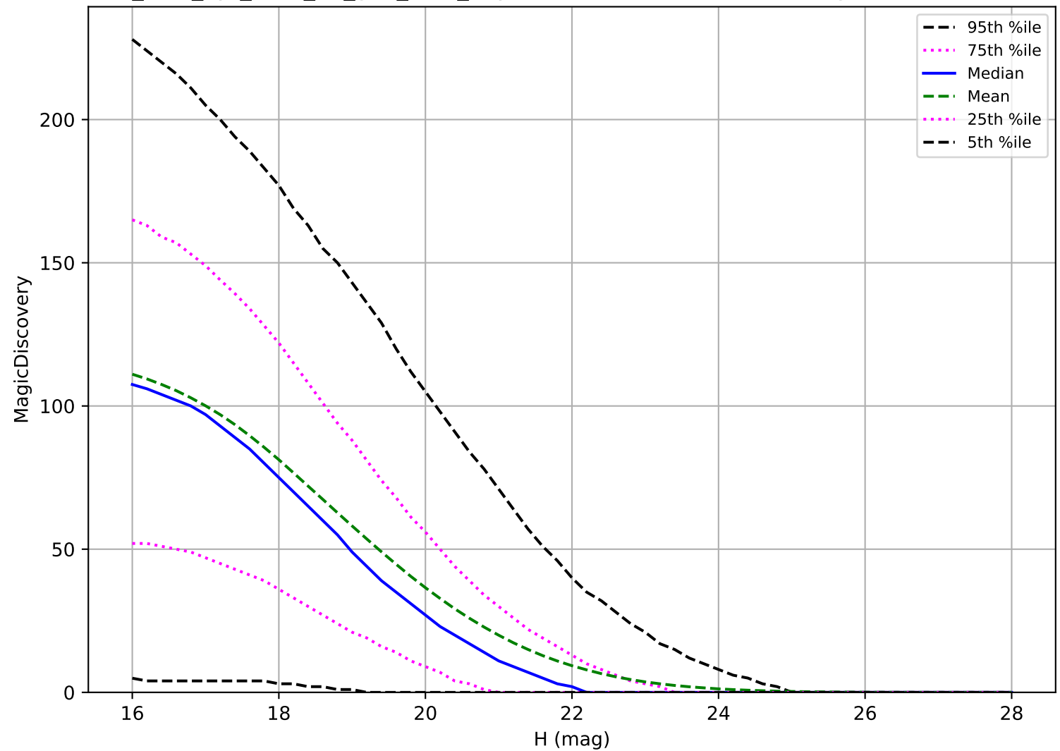
too_elab_2yr_r128_d2_griz_v3.4_10yrs: NEO 6 detections in 60 nights detection loss
