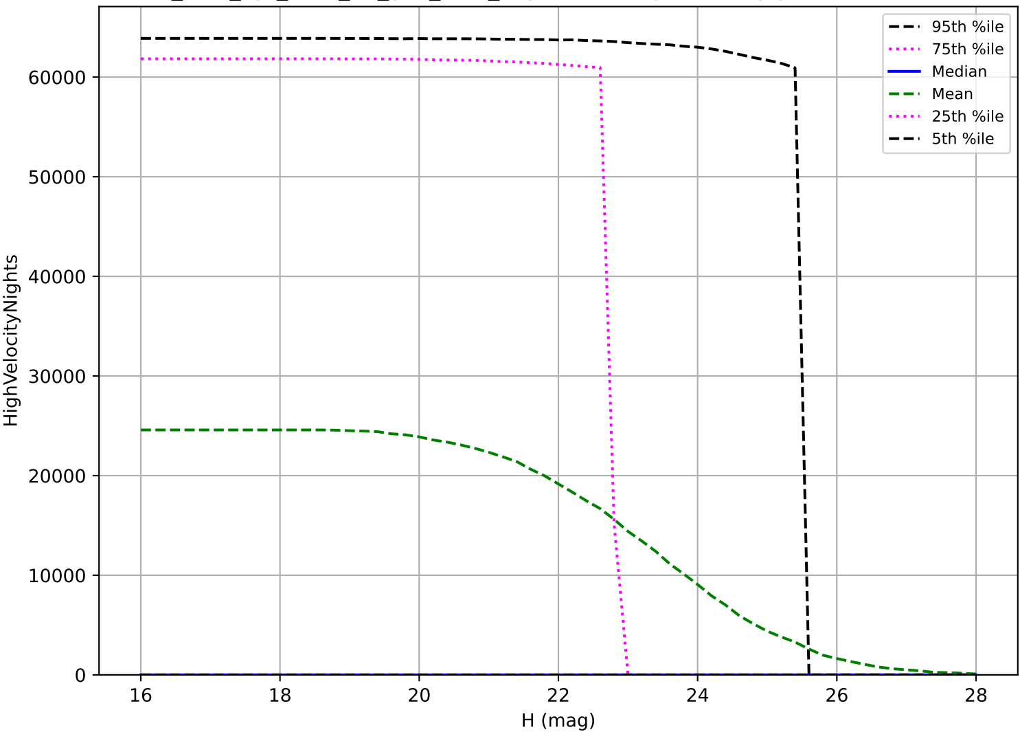
too_elab_2yr_r128_d2_griz_v3.4_10yrs: PHA High velocity pair detection loss
