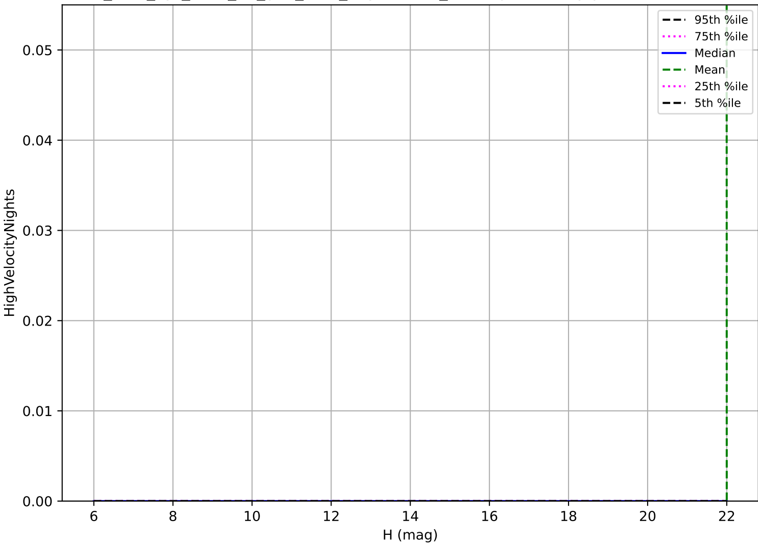
too_elab_2yr_r128_d2_griz_v3.4_10yrs: OCC_r20 High velocity pair detection loss
