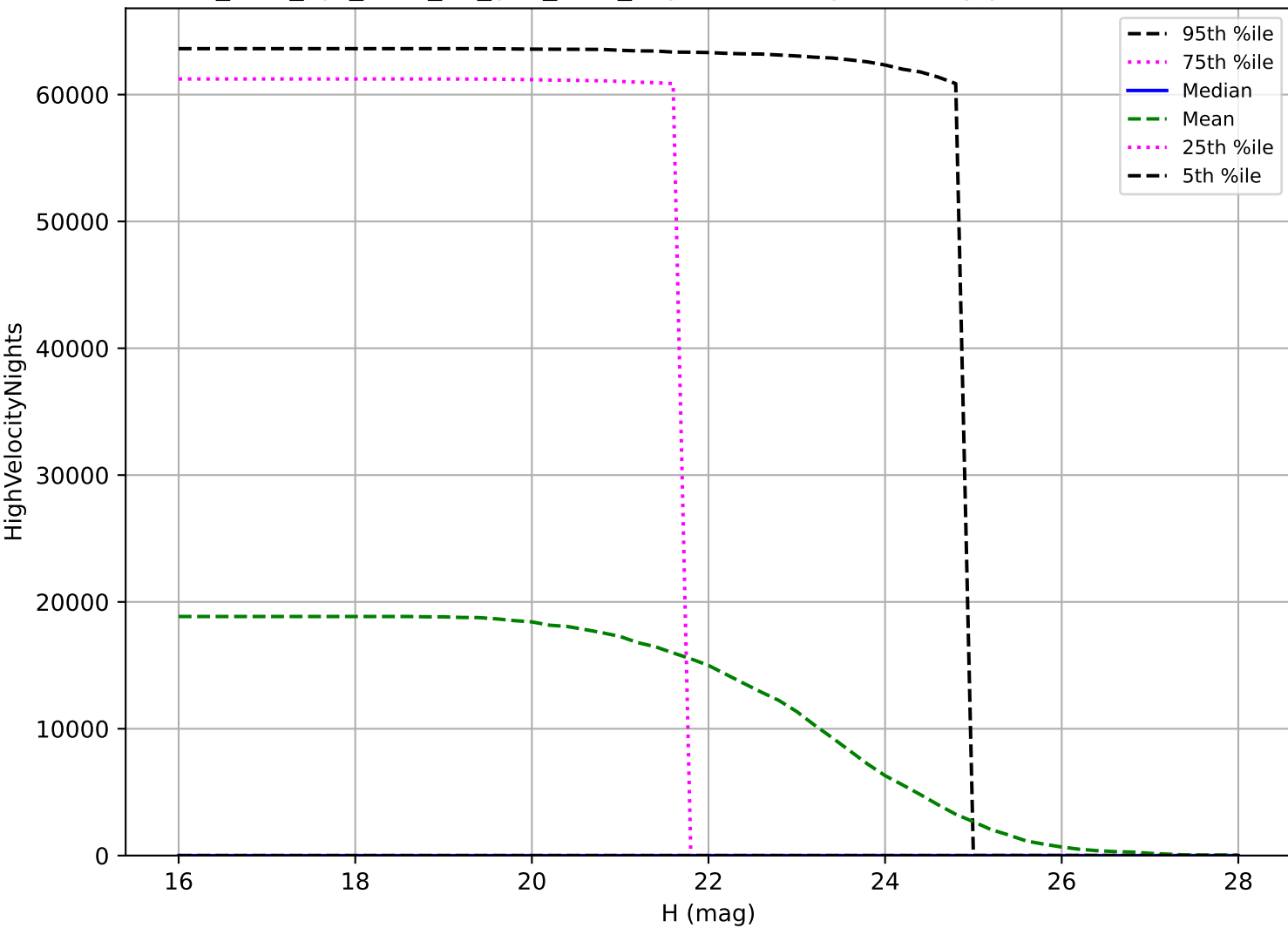
too_elab_2yr_r128_d2_griz_v3.4_10yrs: NEO High velocity pair detection loss
