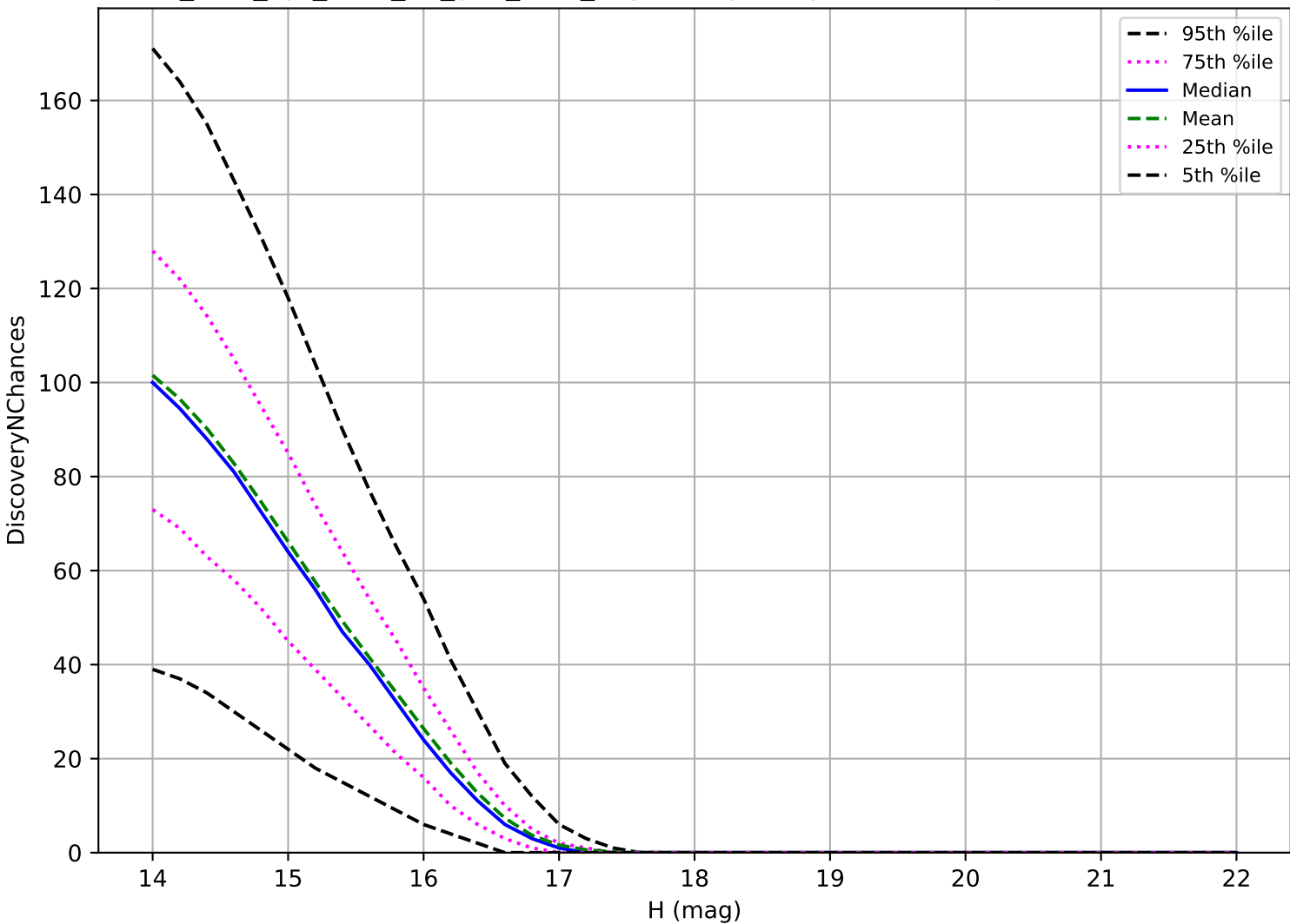
too_elab_2yr_r128_d2_griz_v3.4_10yrs: Trojan 3 pairs in 15 nights detection loss
