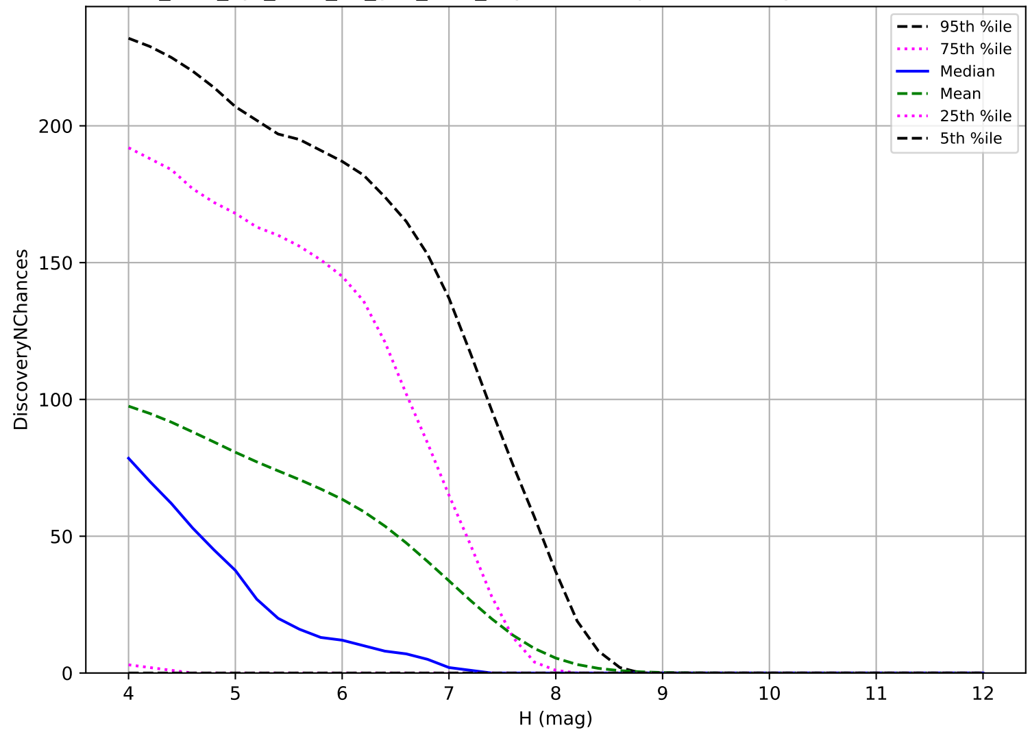
too_elab_2yr_r128_d2_griz_v3.4_10yrs: TNO 3 pairs in 15 nights detection loss
