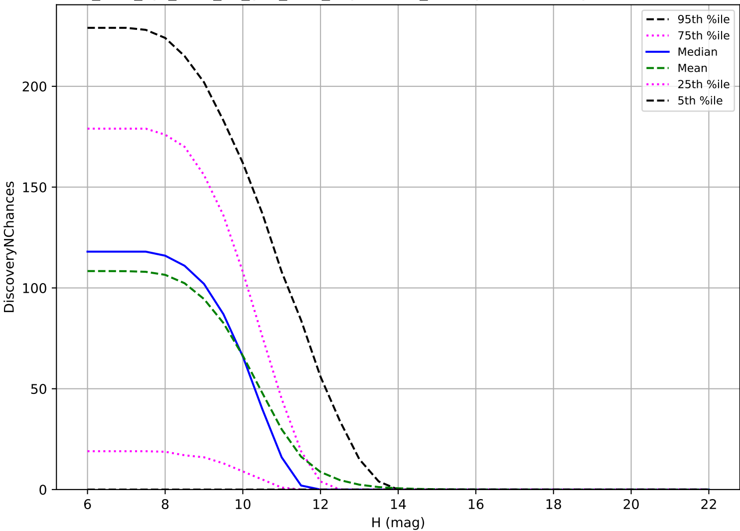
too_elab_2yr_r128_d2_griz_v3.4_10yrs: OCC_r20 3 pairs in 15 nights detection loss
