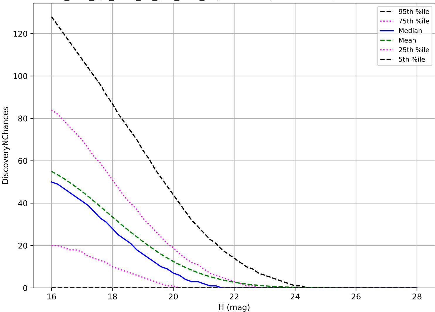
too_elab_2yr_r128_d2_griz_v3.4_10yrs: NEO 3 pairs in 15 nights detection loss
