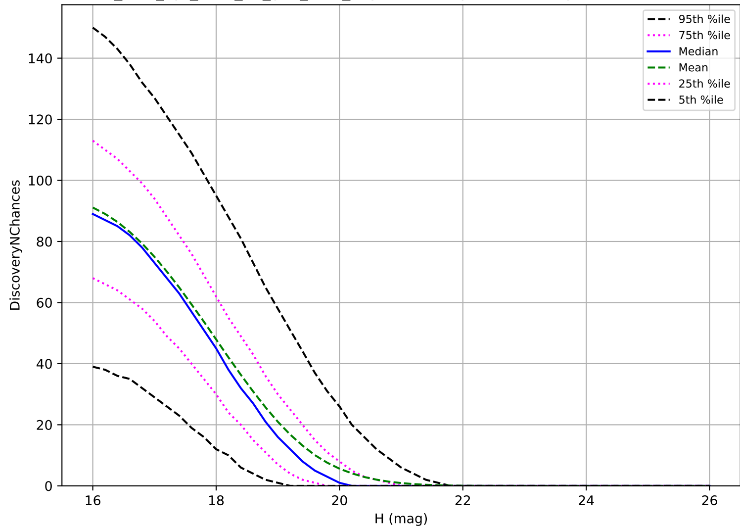
too_elab_2yr_r128_d2_griz_v3.4_10yrs: MBA 3 pairs in 15 nights detection loss
