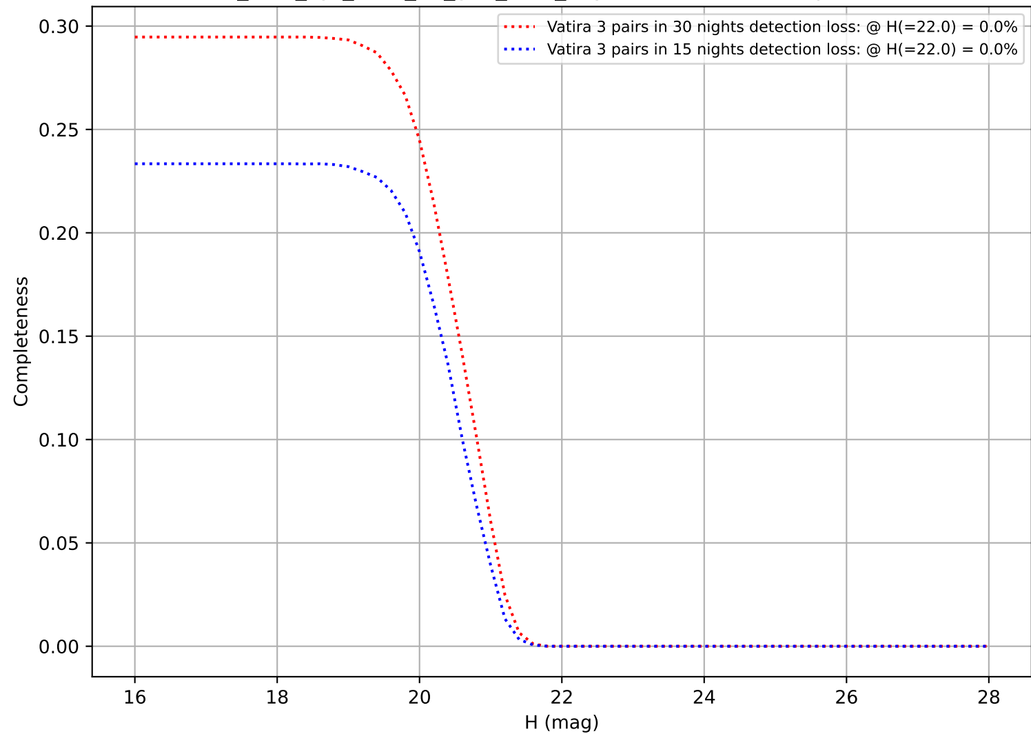
too_elab_2yr_r128_d2_griz_v3.4_10yrs: DifferentialCompleteness
