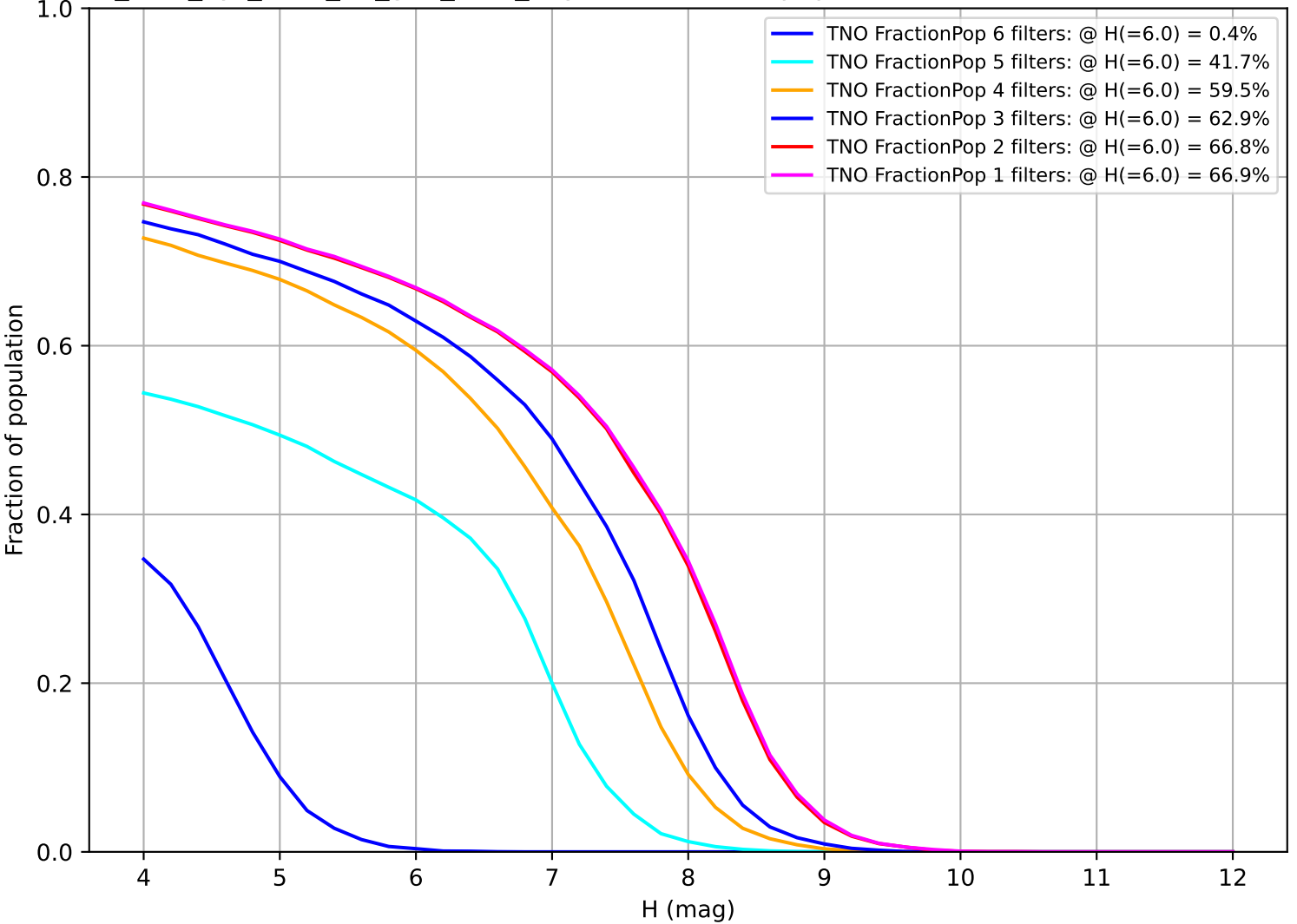
too_elab_2yr_r128_d2_griz_v3.4_10yrs: Fraction of population with colors in X filters TNO
