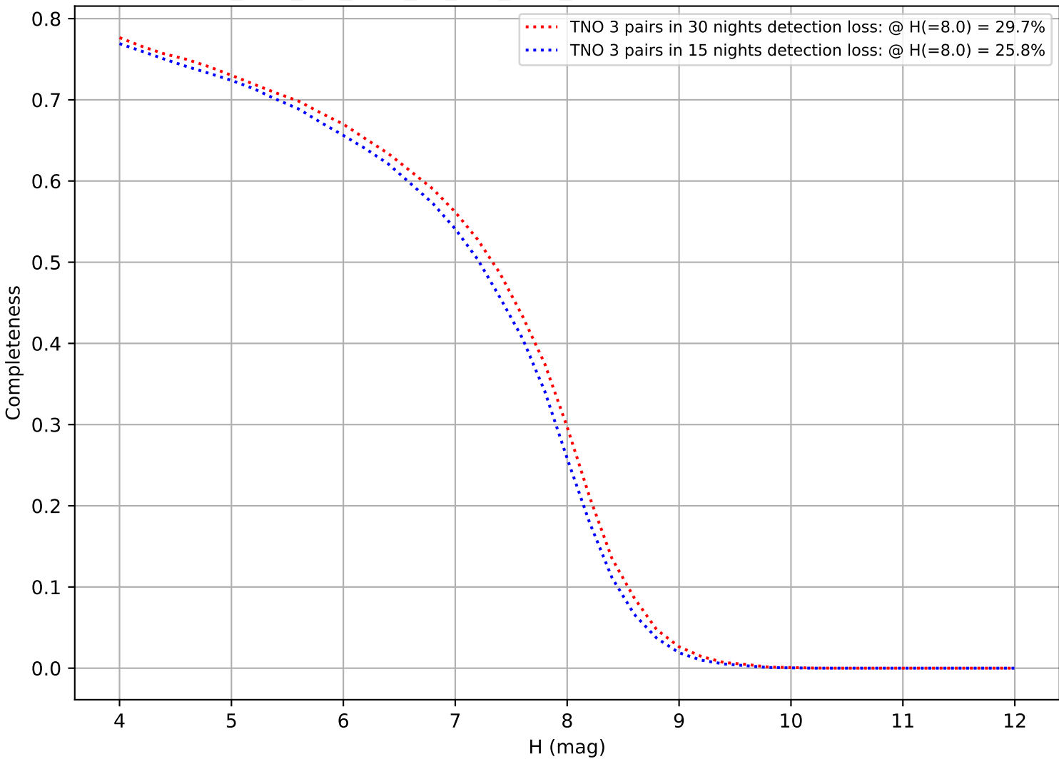
too_elab_2yr_r128_d2_griz_v3.4_10yrs: DifferentialCompleteness
