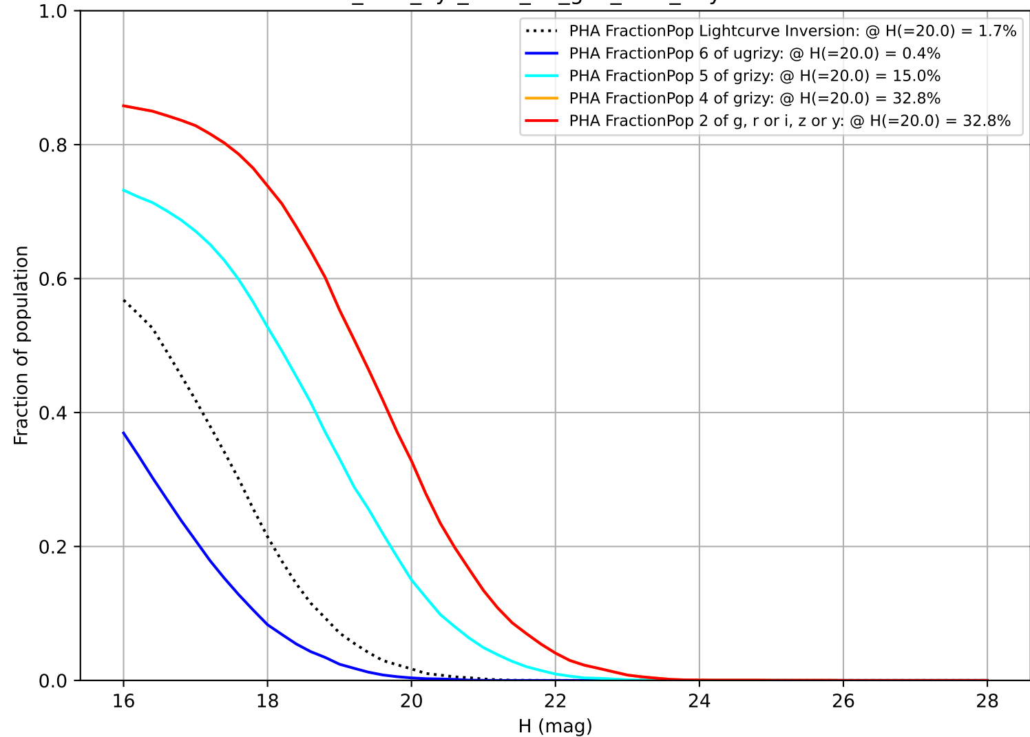
too_elab_2yr_r128_d2_griz_v3.4_10yrs PHA
