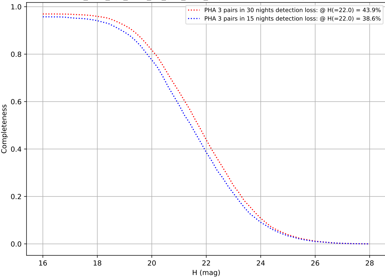
too_elab_2yr_r128_d2_griz_v3.4_10yrs: DifferentialCompleteness
