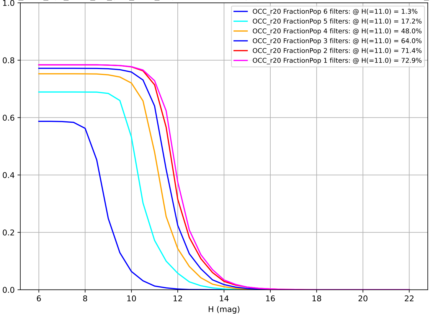
too_elab_2yr_r128_d2_griz_v3.4_10yrs: Fraction of population with colors in X filters OCC_r20
