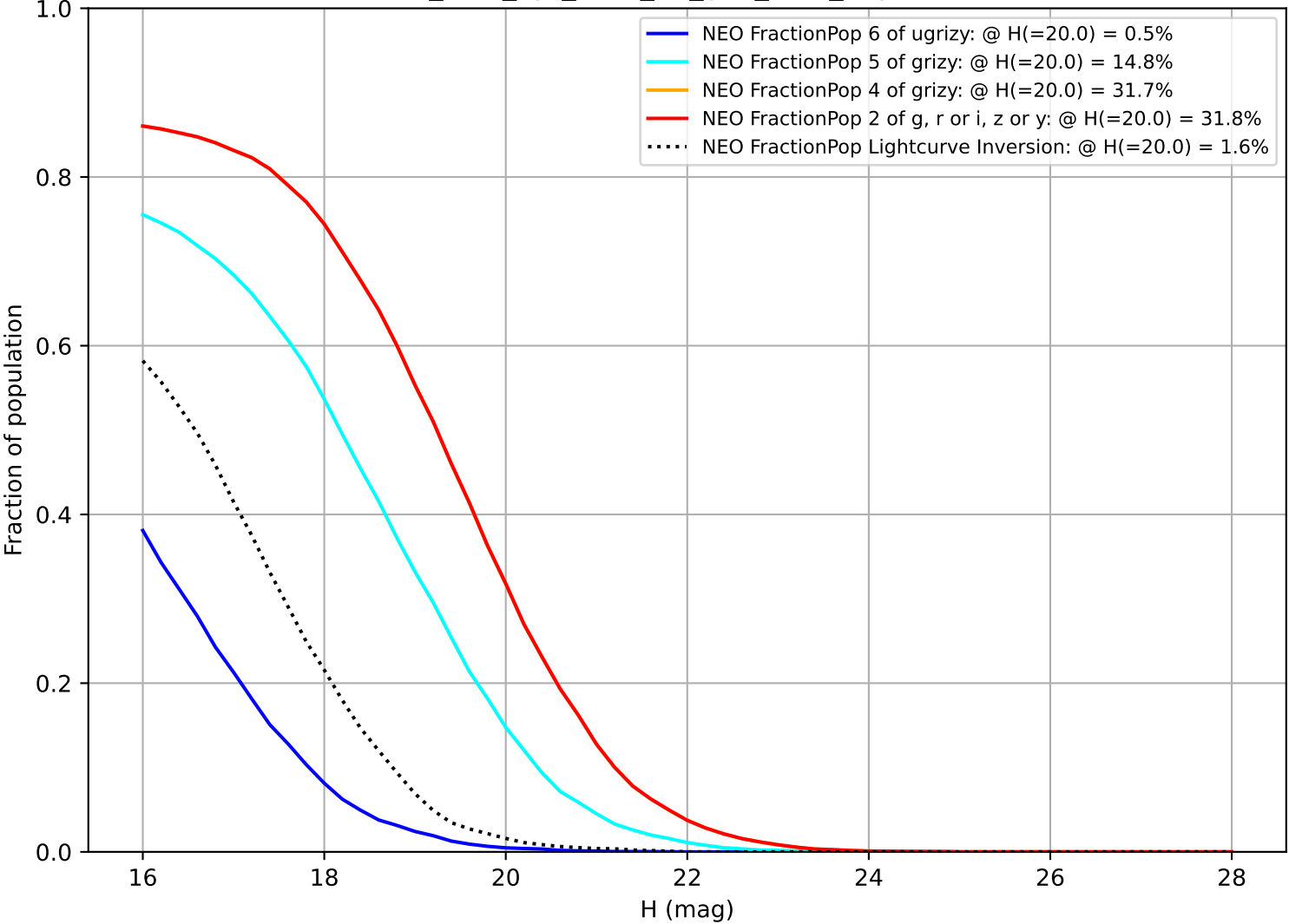
too_elab_2yr_r128_d2_griz_v3.4_10yrs NEO
