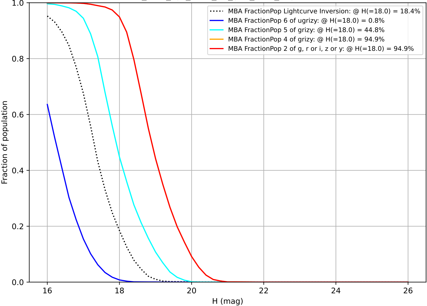
too_elab_2yr_r128_d2_griz_v3.4_10yrs MBA
