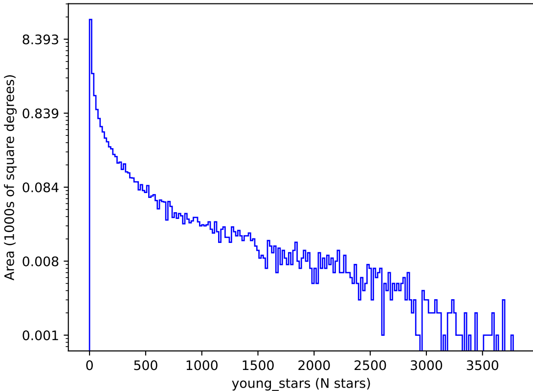
too_elab_2yr_r128_d2_griz_v3.4_10yrs : young_stars
