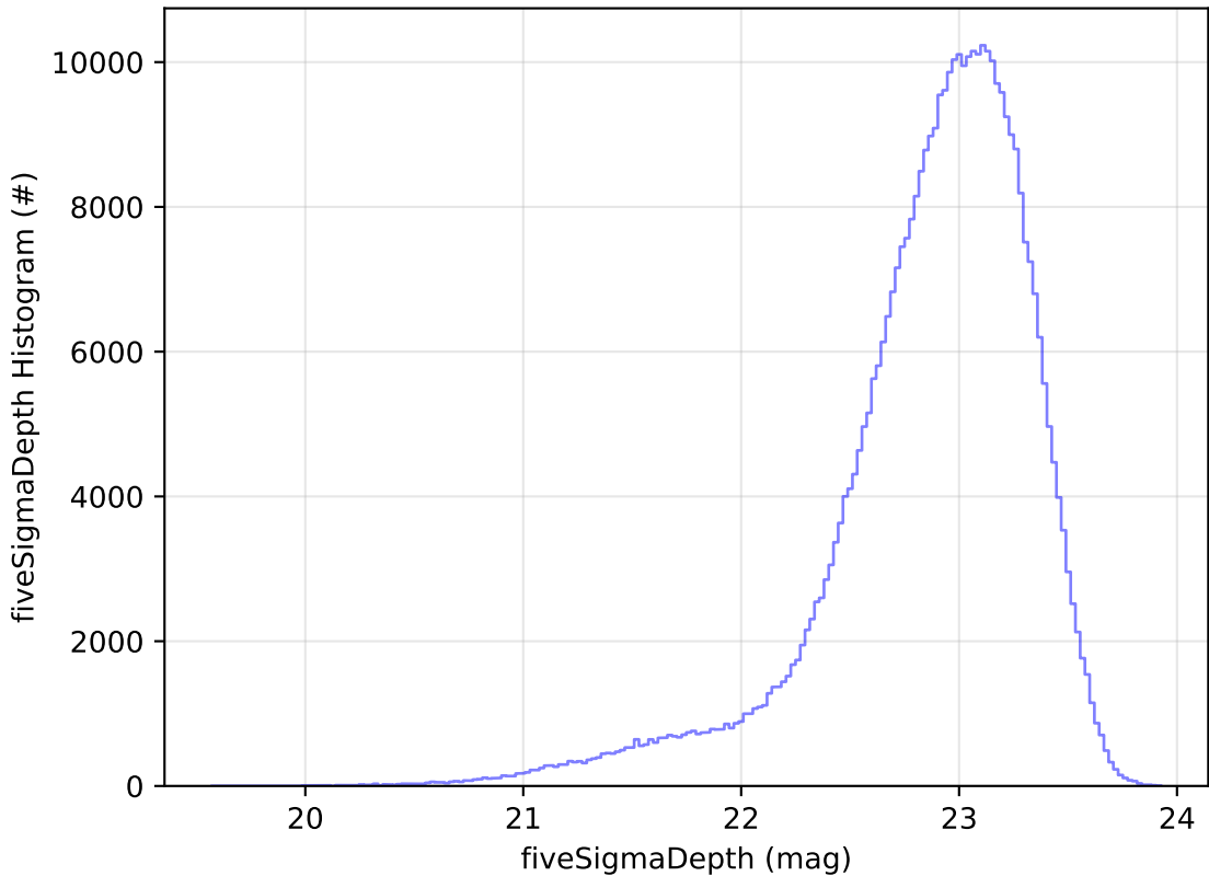
too_elab_2yr_r128_d2_griz_v3.4_10yrs z: fiveSigmaDepth Histogram
