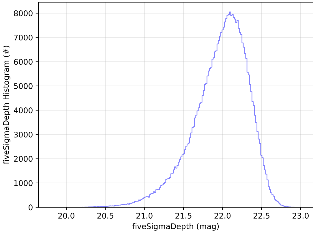
too_elab_2yr_r128_d2_griz_v3.4_10yrs y: fiveSigmaDepth Histogram
