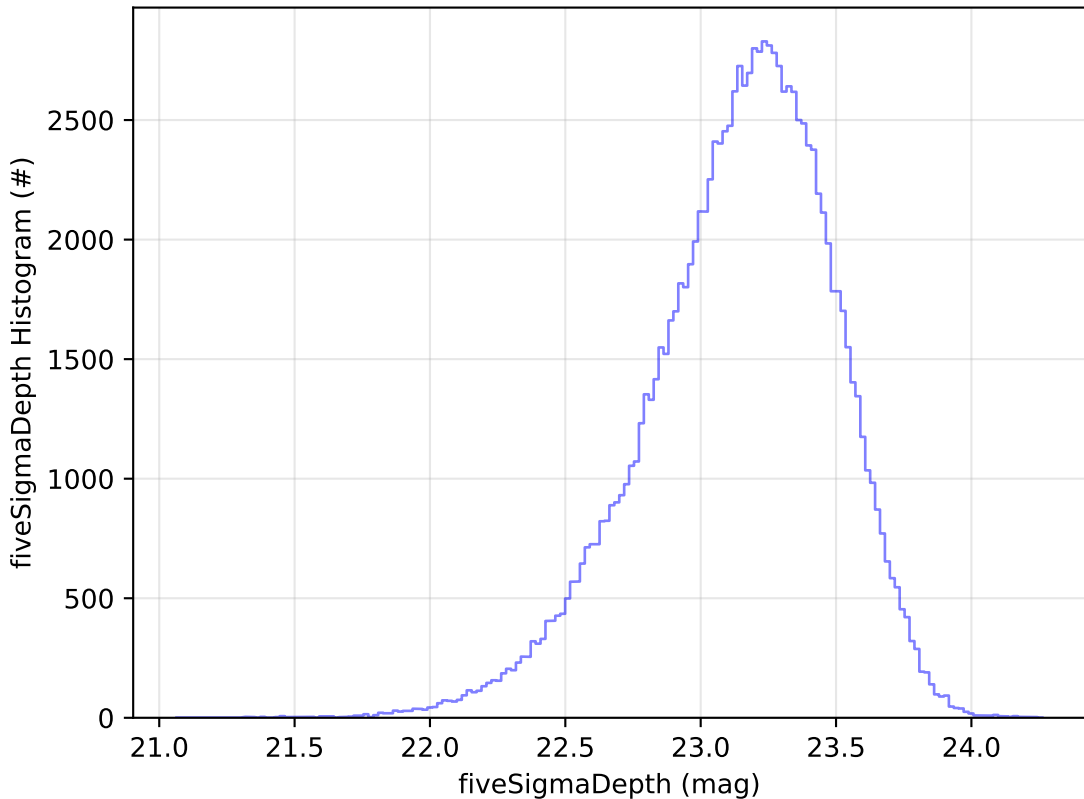
too_elab_2yr_r128_d2_griz_v3.4_10yrs u: fiveSigmaDepth Histogram
