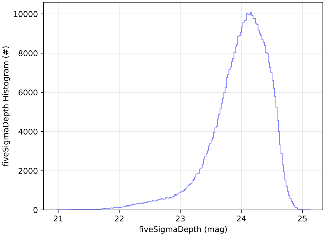
too_elab_2yr_r128_d2_griz_v3.4_10yrs r: fiveSigmaDepth Histogram
