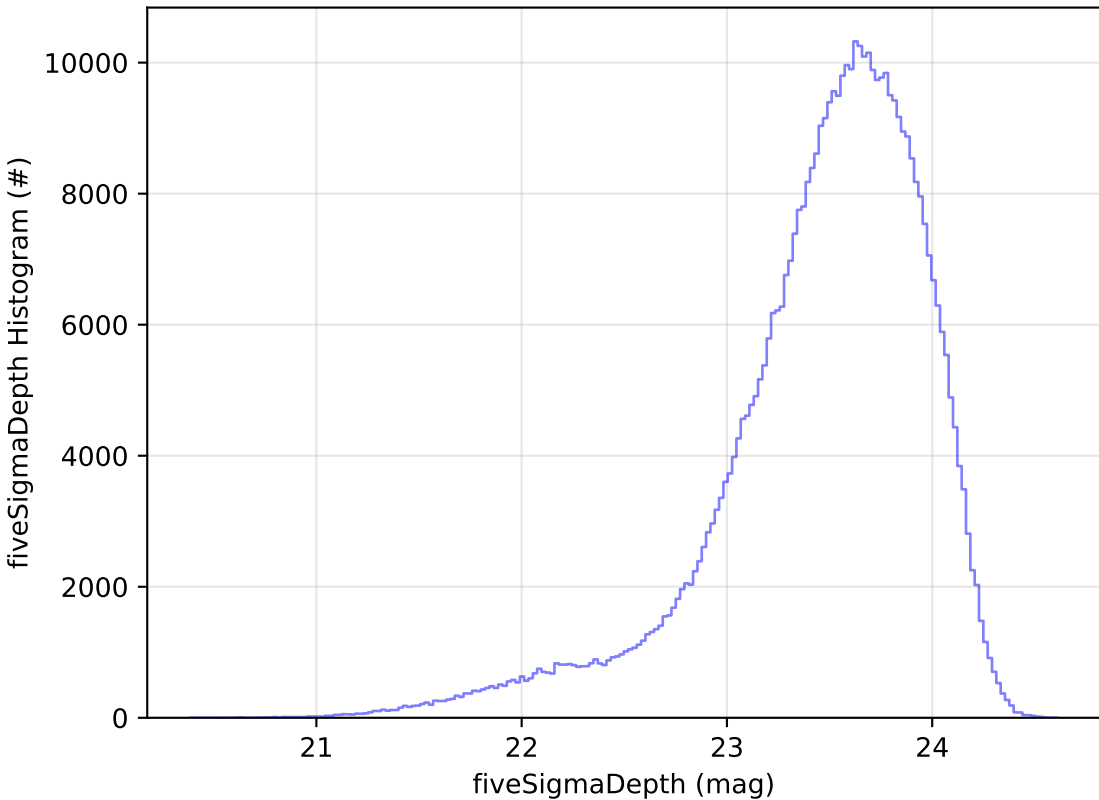
too_elab_2yr_r128_d2_griz_v3.4_10yrs i: fiveSigmaDepth Histogram
