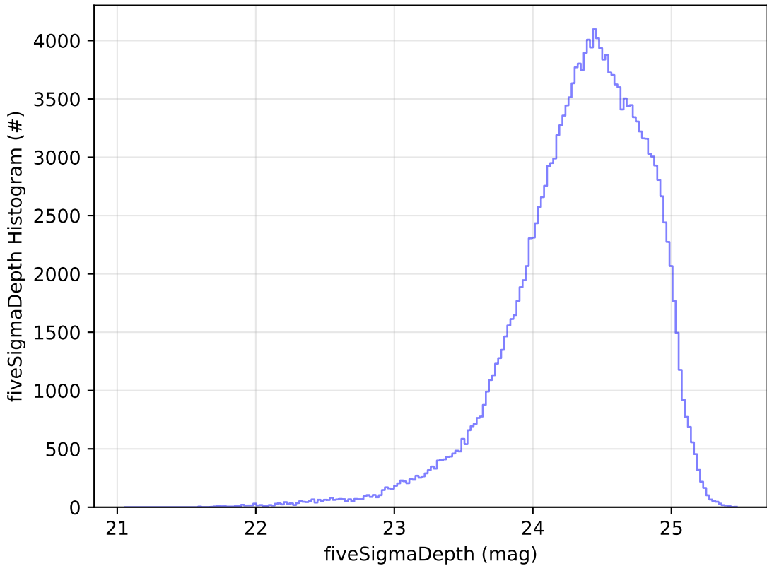
too_elab_2yr_r128_d2_griz_v3.4_10yrs g: fiveSigmaDepth Histogram
