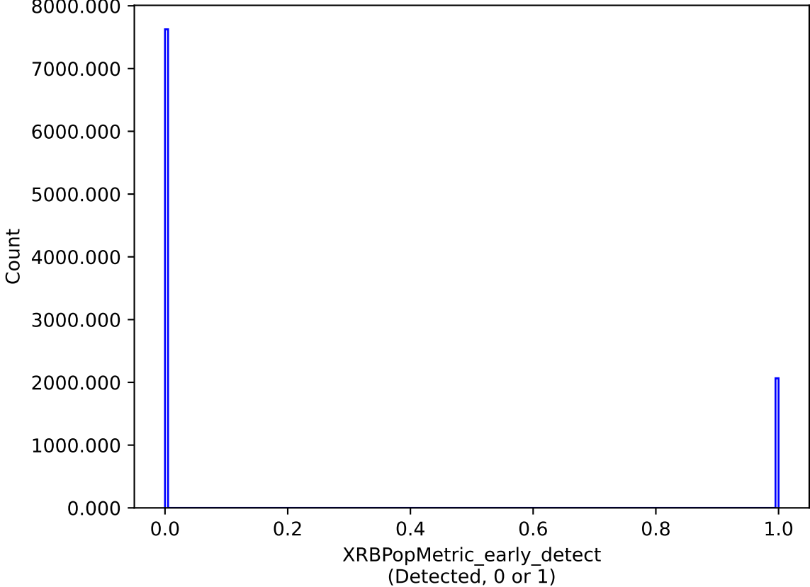
too_elab_2yr_r128_d2_griz_v3.4_10yrs : XRBPopMetric_early_detect
