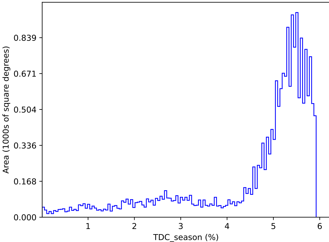
too_elab_2yr_r128_d2_griz_v3.4_10yrs : TDC_season
