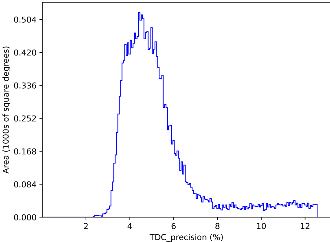
too_elab_2yr_r128_d2_griz_v3.4_10yrs : TDC_precision
