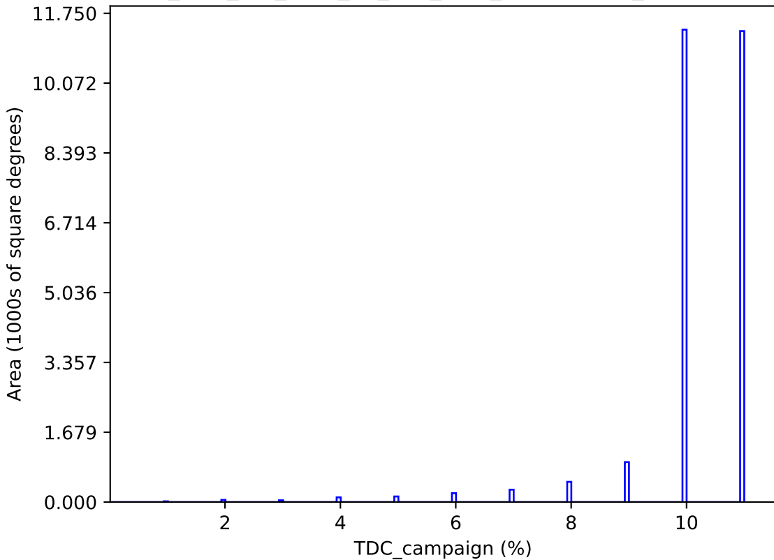
too_elab_2yr_r128_d2_griz_v3.4_10yrs : TDC_campaign
