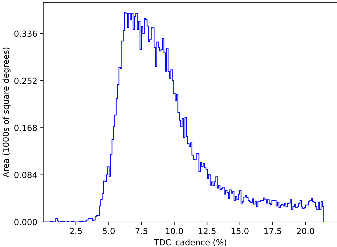
too_elab_2yr_r128_d2_griz_v3.4_10yrs : TDC_cadence
