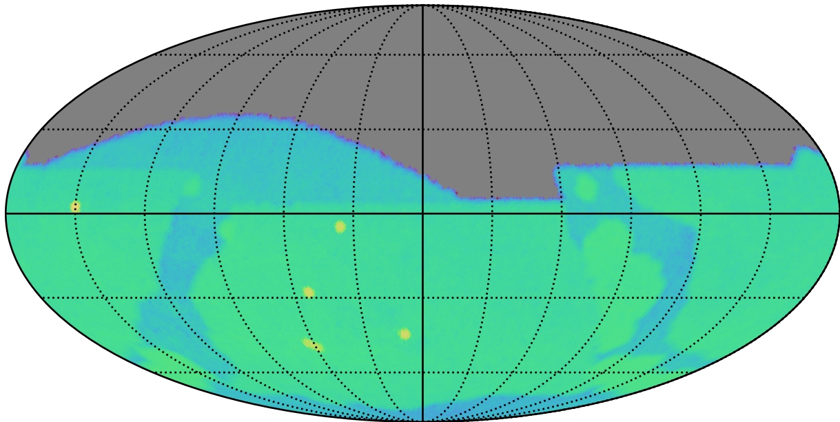
too_elab_2yr_r128_d2_griz_v3.4_10yrs g: SurfaceBrightLimit
