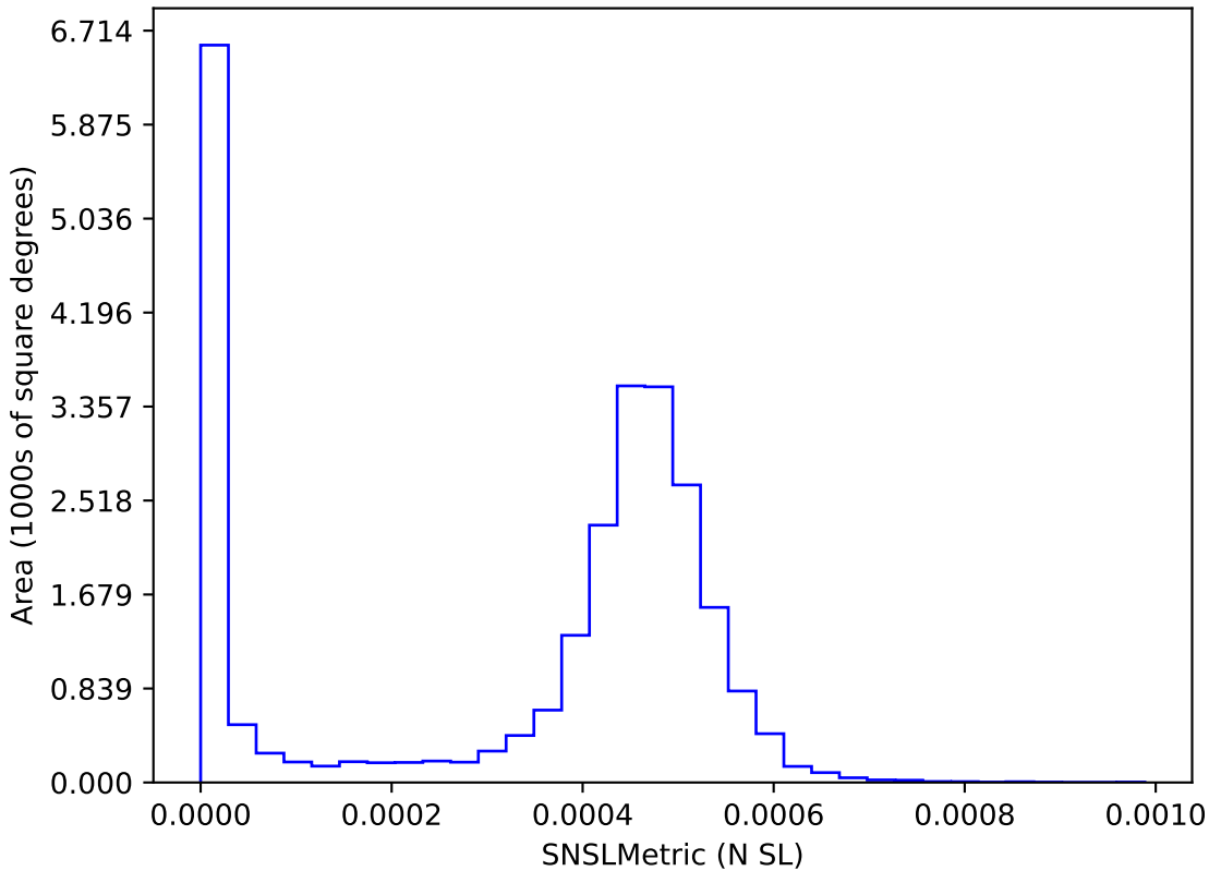
too_elab_2yr_r128_d2_griz_v3.4_10yrs : SNSLMetric
