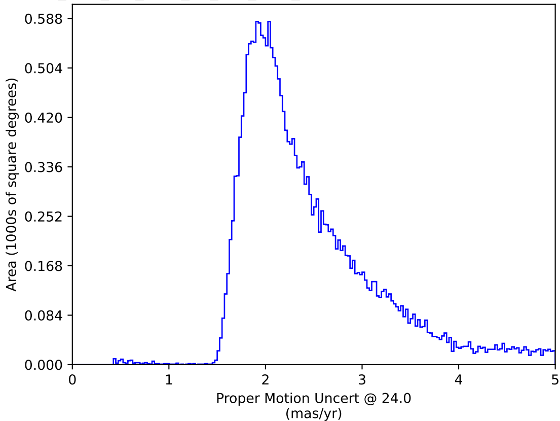
too_elab_2yr_r128_d2_griz_v3.4_10yrs : Proper Motion Uncert @ 24.0
