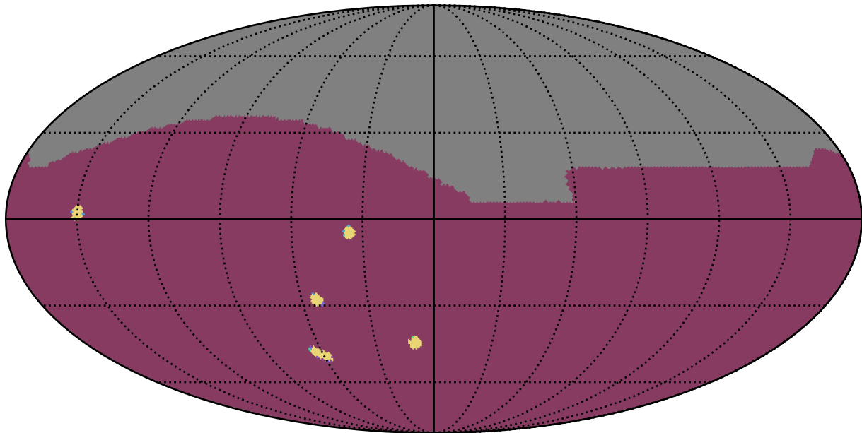
too_elab_2yr_r128_d2_griz_v3.4_10yrs : NumberOfQuickRevisits
