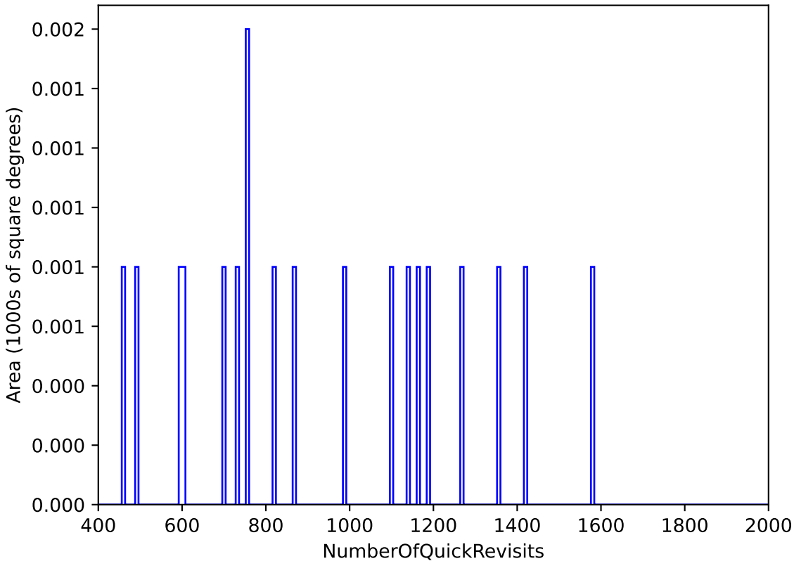
too_elab_2yr_r128_d2_griz_v3.4_10yrs : NumberOfQuickRevisits
