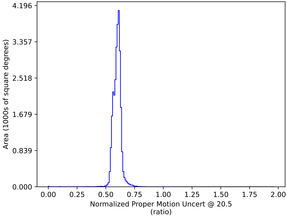
too_elab_2yr_r128_d2_griz_v3.4_10yrs : Normalized Proper Motion Uncert @ 20.5
