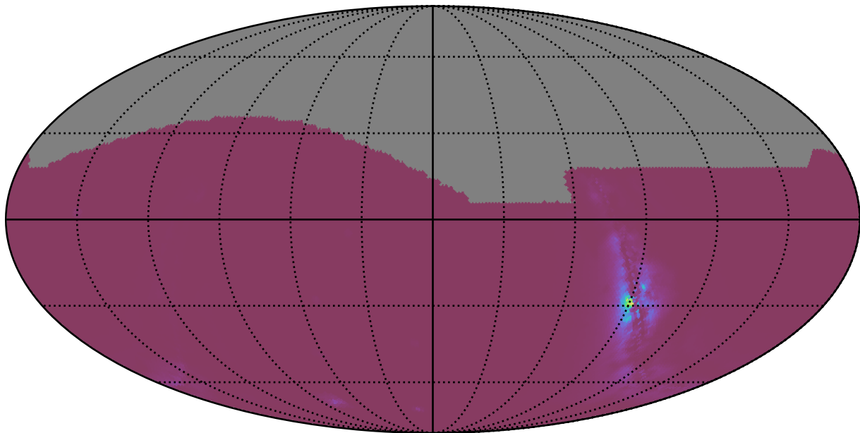
too_elab_2yr_r128_d2_griz_v3.4_10yrs : NlcPoints
