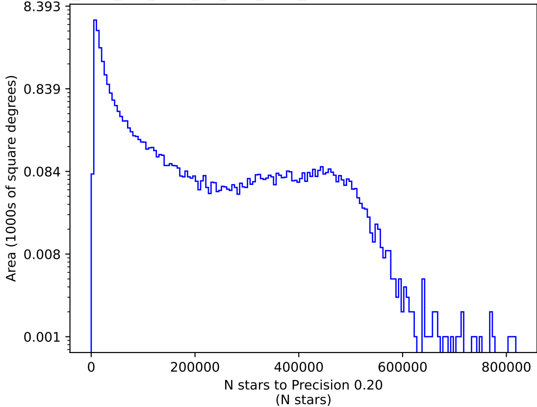
too_elab_2yr_r128_d2_griz_v3.4_10yrs i: N stars to Precision 0.20
