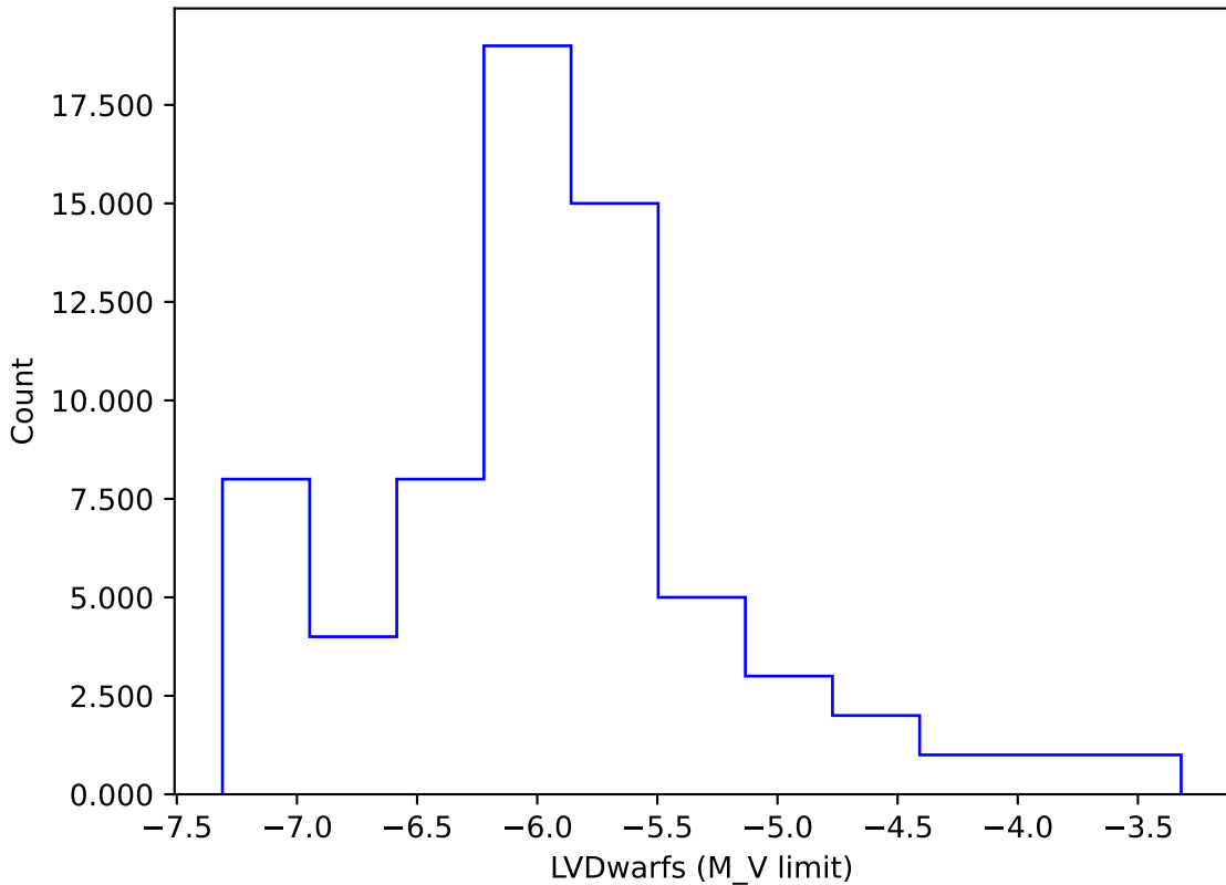
too_elab_2yr_r128_d2_griz_v3.4_10yrs gi: LVDwarfs
