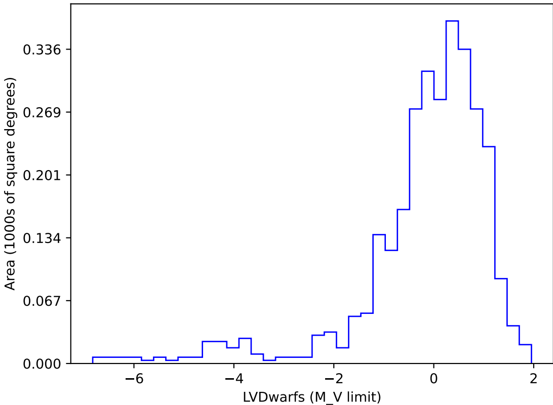
too_elab_2yr_r128_d2_griz_v3.4_10yrs gi SCP: LVDwarfs
