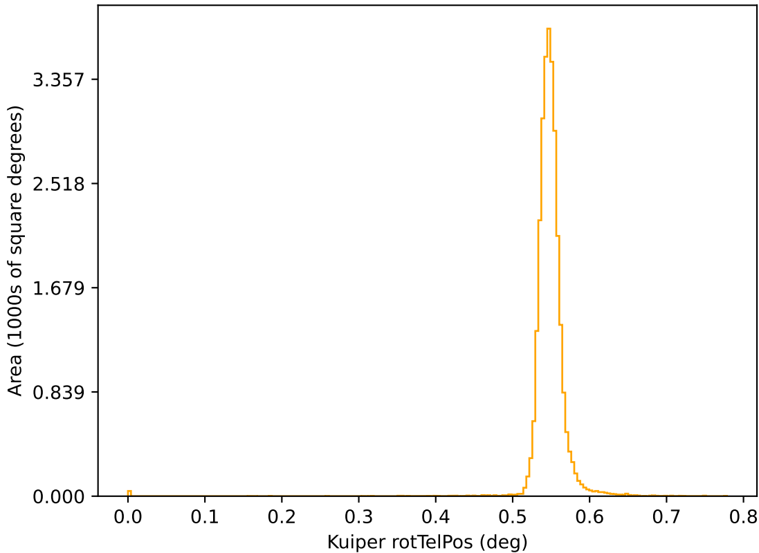
too_elab_2yr_r128_d2_griz_v3.4_10yrs r: Kuiper rotTelPos
