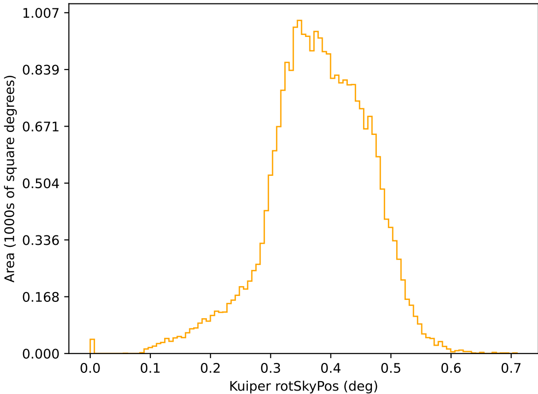
too_elab_2yr_r128_d2_griz_v3.4_10yrs r: Kuiper rotSkyPos
