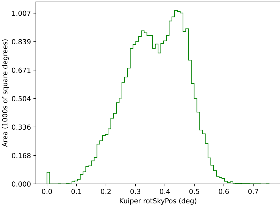
too_elab_2yr_r128_d2_griz_v3.4_10yrs g: Kuiper rotSkyPos
