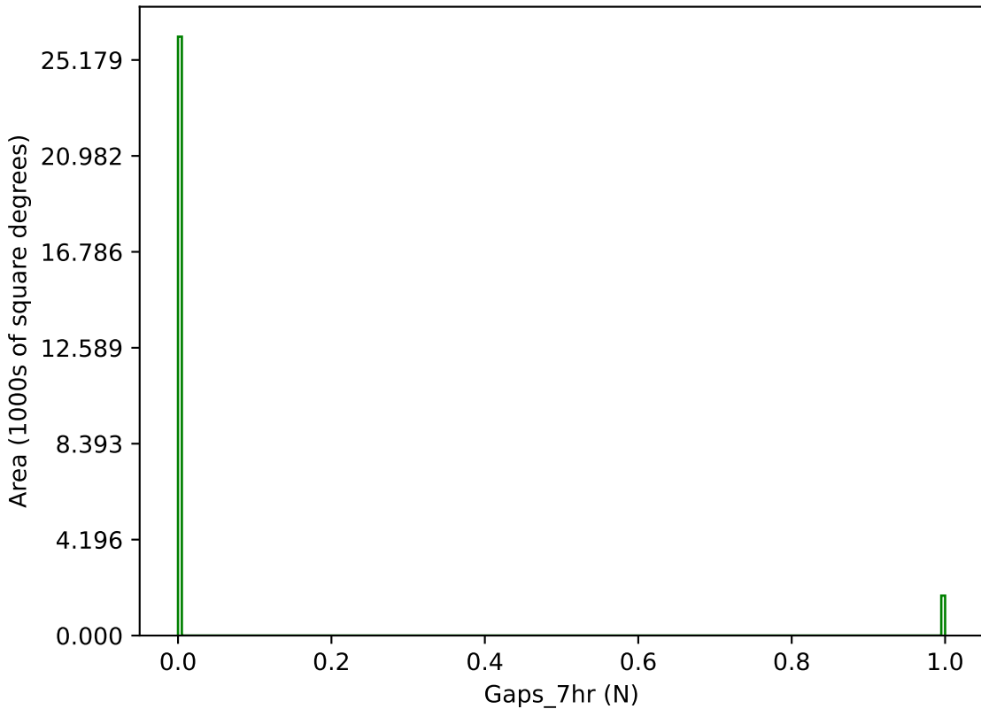
too_elab_2yr_r128_d2_griz_v3.4_10yrs g band: Gaps_7hr
