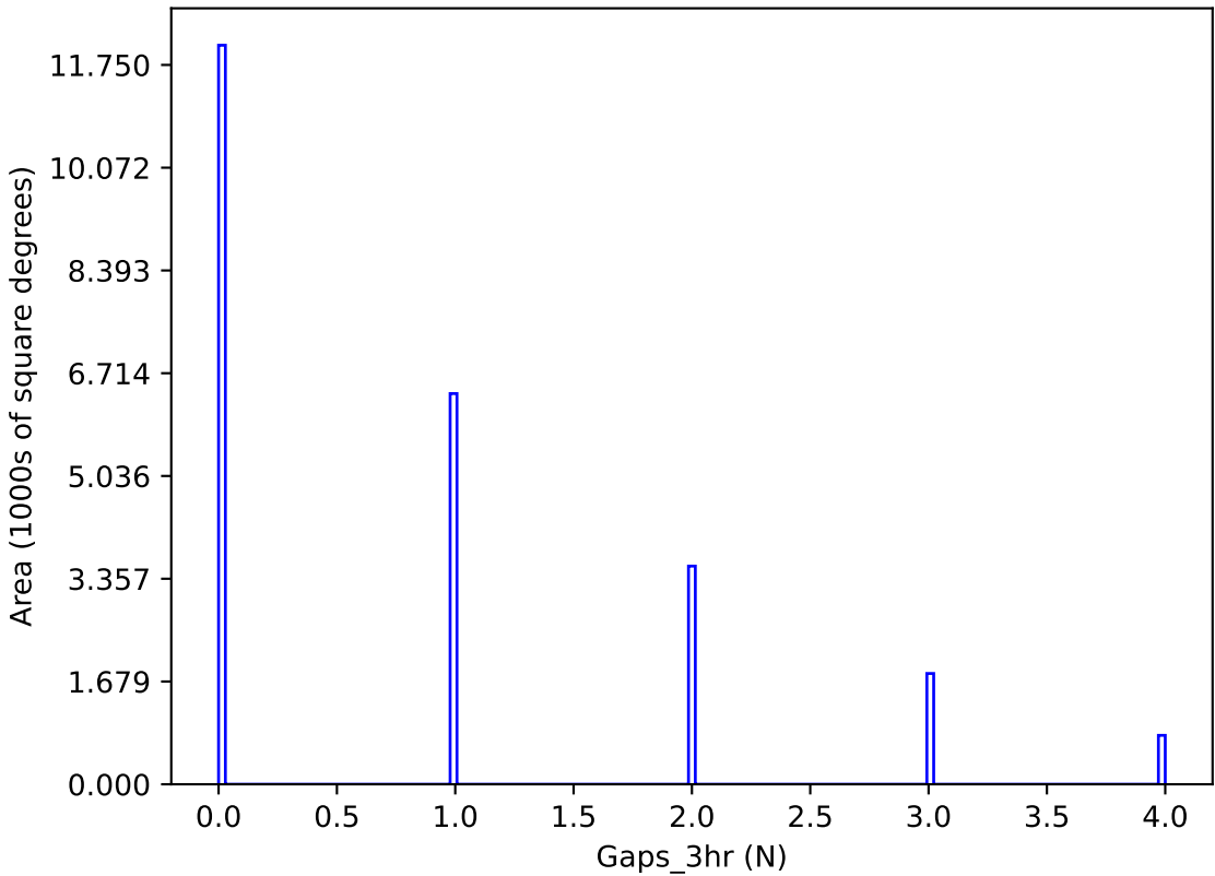
too_elab_2yr_r128_d2_griz_v3.4_10yrs y band: Gaps_3hr
