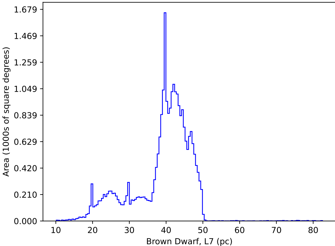
too_elab_2yr_r128_d2_griz_v3.4_10yrs : Brown Dwarf, L7
