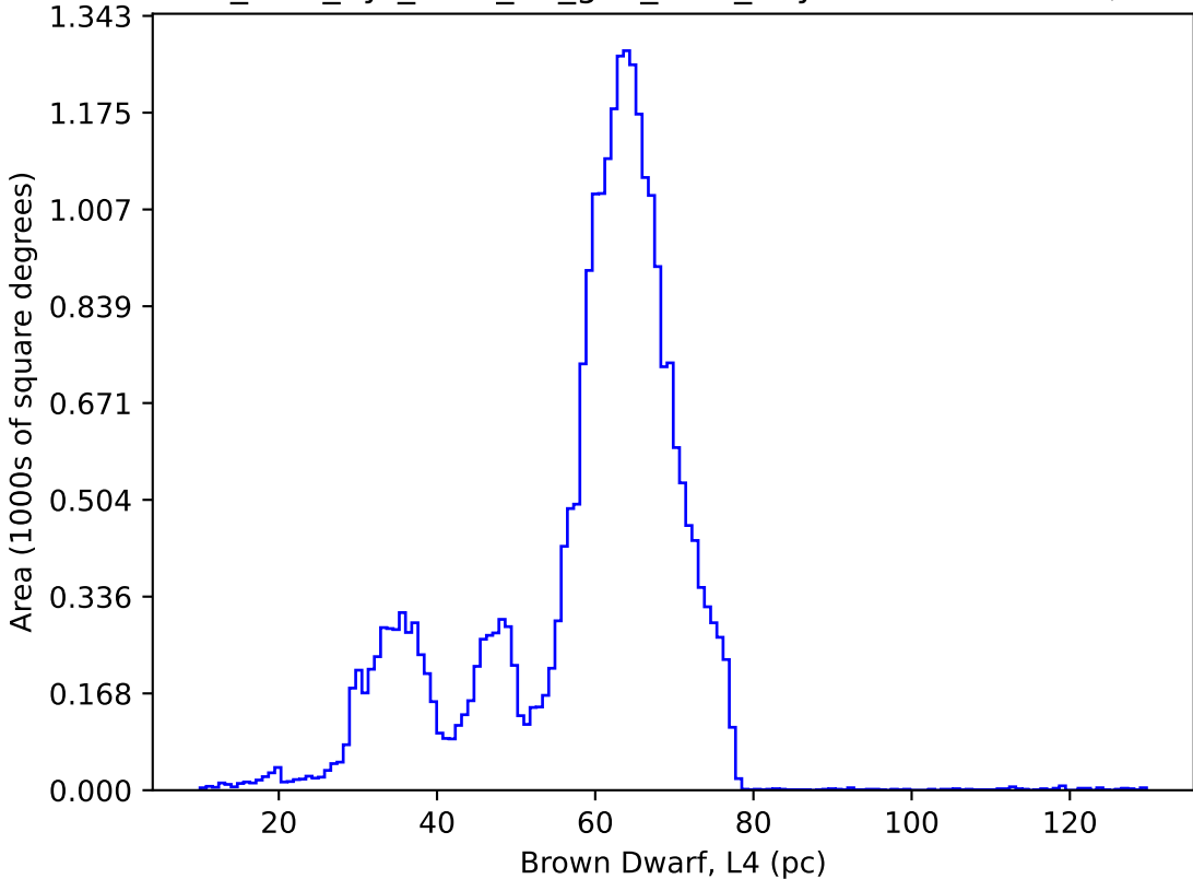
too_elab_2yr_r128_d2_griz_v3.4_10yrs : Brown Dwarf, L4
