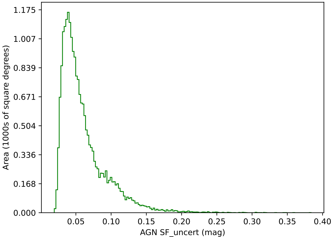
too_elab_2yr_r128_d2_griz_v3.4_10yrs g band: AGN SF_uncert
