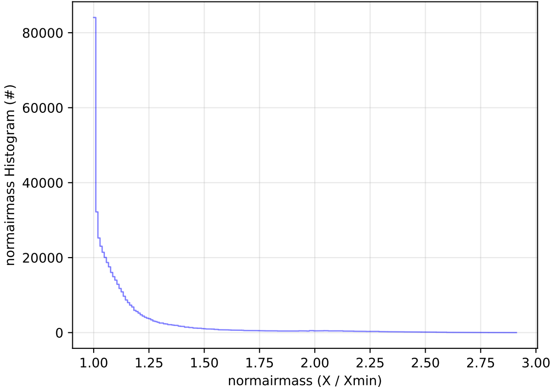
too_elab_2yr_r128_d2_griz_v3.4_10yrs All sky i band: normairmass Histogram
